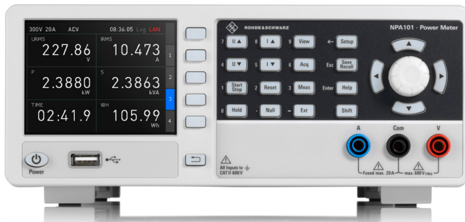
R&S®NPA101
