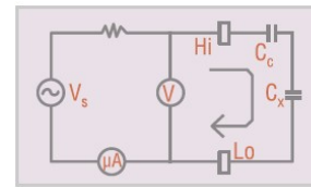
回路開放時： C_m = C_c * C_x / (C_c + C_x) \ll C_x
