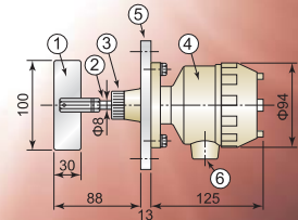
NL-8B (接粉部SUS)
